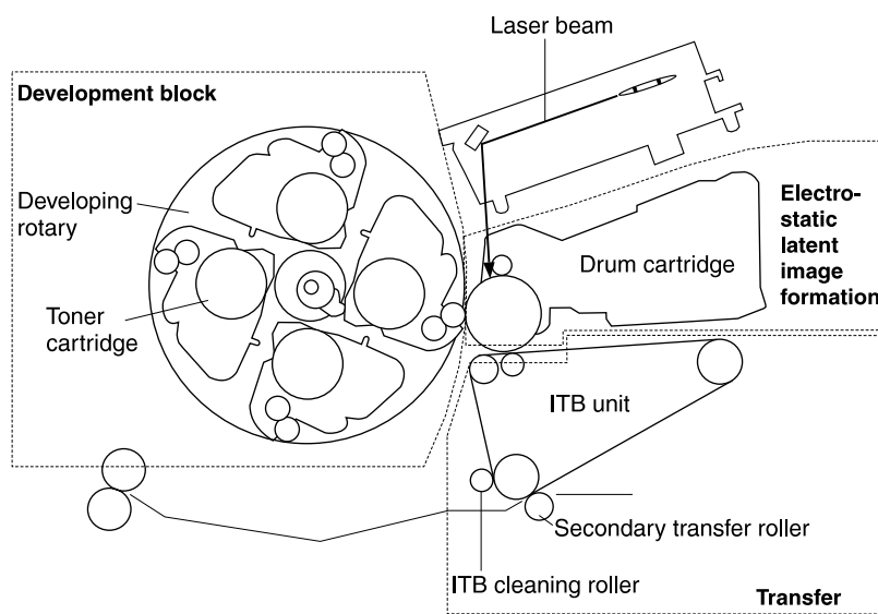
Figure 7-6 Image formation
