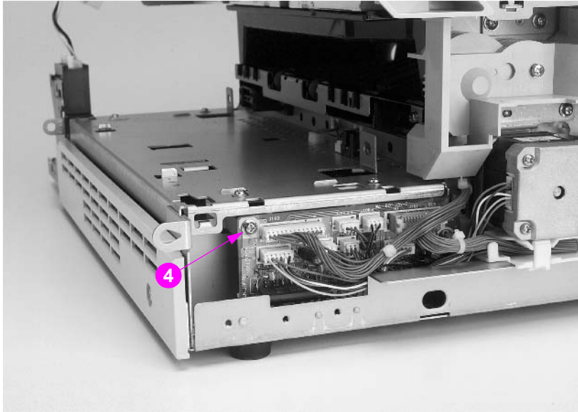
Figure 6-46 Paper feed PCB removal and replacement (3 of 3)
