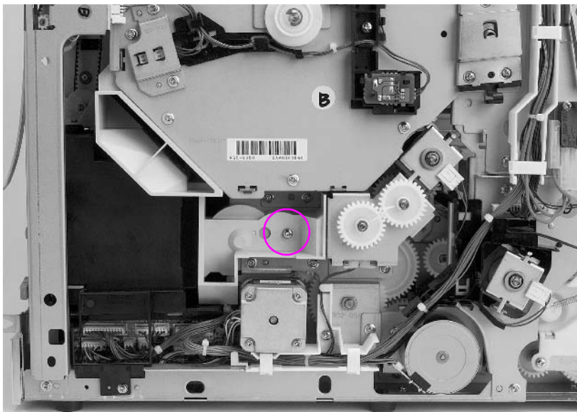
Figure 6-52 ITB clutch assembly removal and replacement (1 of 2)
