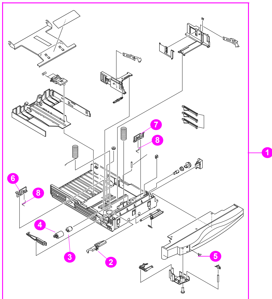
Figure 8-15 250-sheet cassette
