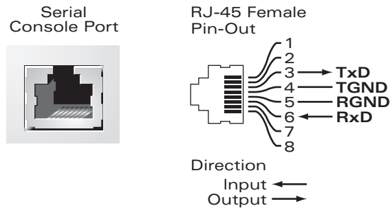
FIGURE B-5 Serial Port
