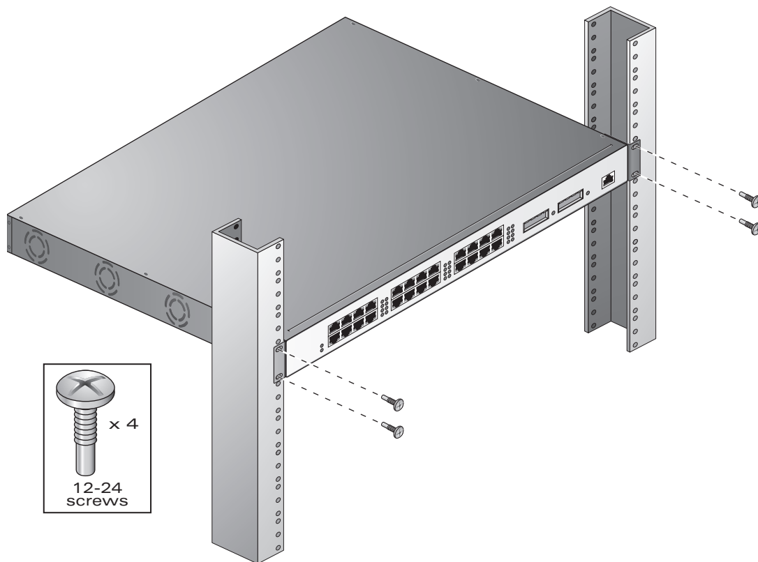
FIGURE 2-3 Mounting the Mobility Controller
