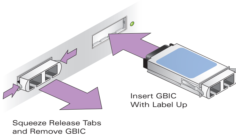
FIGURE B-4 GBIC Removal and Insertion
