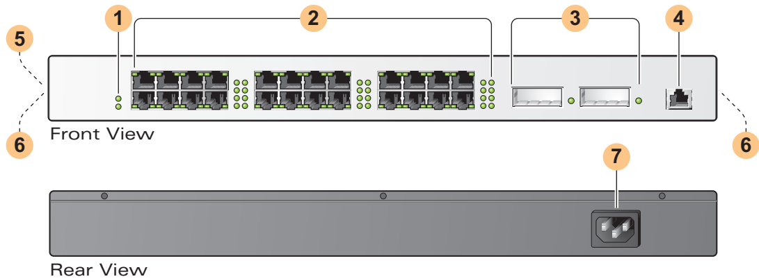
FIGURE 1-1 Aruba 2400 System
