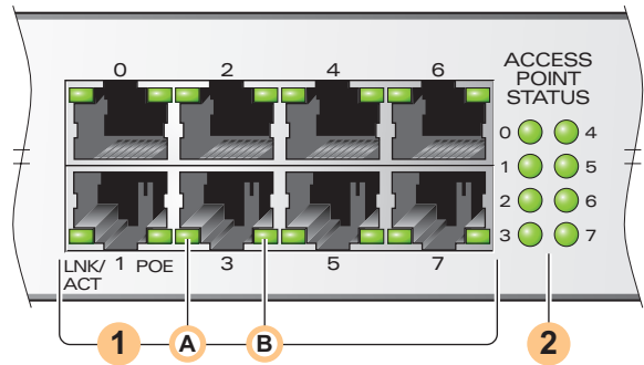
FIGURE B-1 Aruba 2400 FE Network Ports
