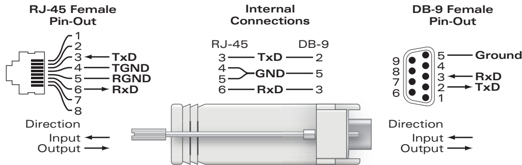
FIGURE B-6 Serial Port Adapter
